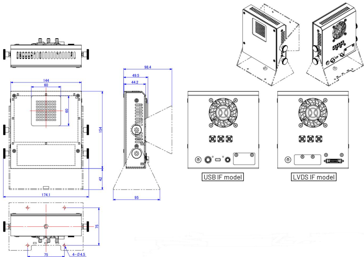
Figure 2 Dragonfly SDK
