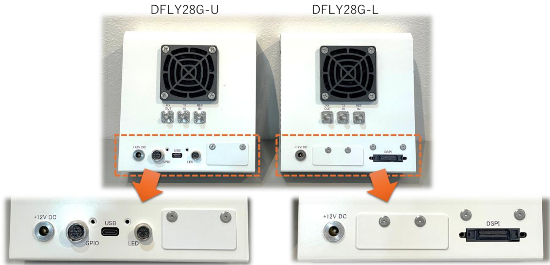
Figure. 5 SDK models
